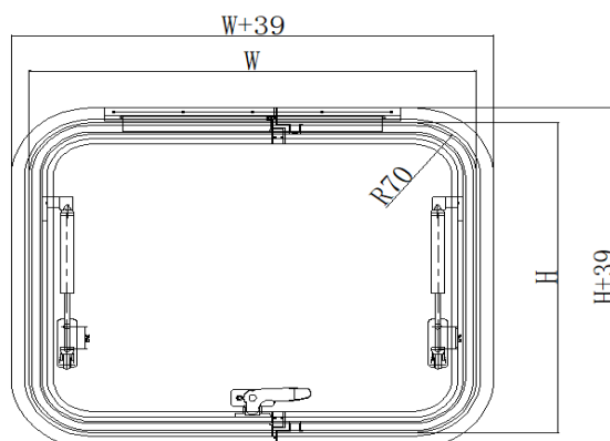
Customizable change of R-angle specifications
