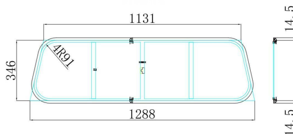
Cutout Size
